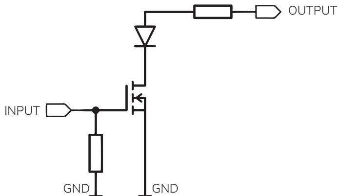
Functional diagram passive output
