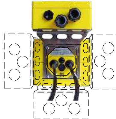
Terminal box mounted beside the actuator
